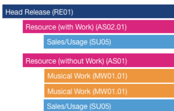
Figure 1 – Two Blocks of Records when Reporting Broadcasts
